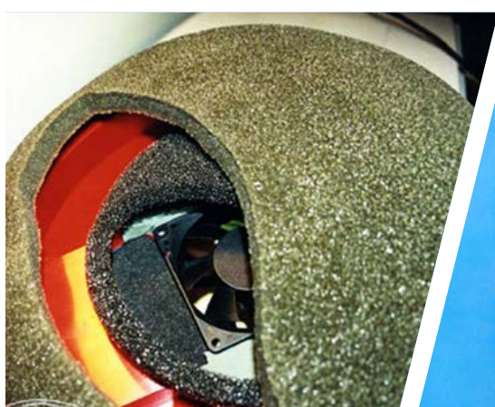
Cutaway section showing outer dust filter, primary filter and inner Carbon filter
